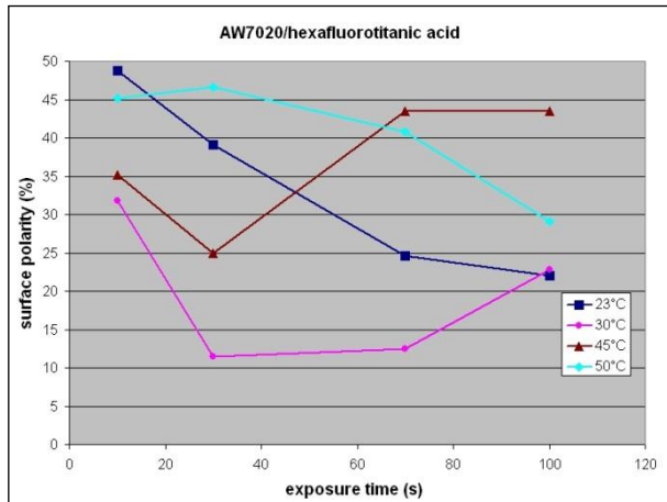
Fig. 2: The surface polarity of sample AW7020 as a function of the exposure time
