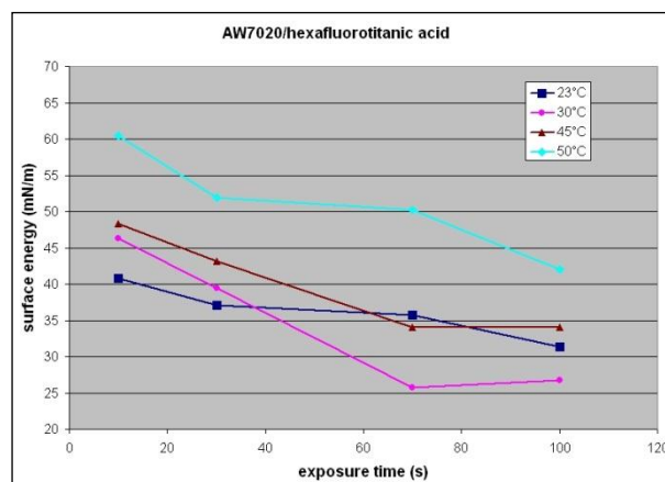
Fig.1b: SFE of AW7020 as a function of the conversion bath exposure time
