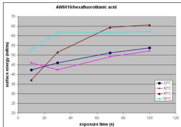
Fig.1a: SFE of AW6016 as a function of the conversion bath exposure time
